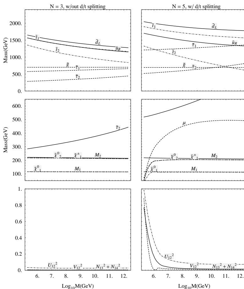
Figure 7: Example spectra with and without doublet/triplet splitting for the type III model (4.5). The left column has N = 3 , \lambda' = 1 , \lambda = 1 , m = X/5 , \Lambda_G = 90 \text{ TeV} , \tan \beta = 20 and \mu > 0 . It shows that a 700 GeV gluino is possible in gauge mediation even keeping the stops heavy for the LEP Higgs mass bound. The right plot has the same parameters, except N = 5 , \lambda_2 = 1 , \lambda_3 = 1/5 . Here we see that a light gluino and a Higgsino NLSP are simultaneously possible, at low messenger scales.
